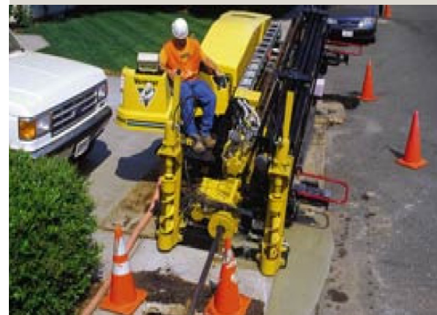
Directional drilling minimizes impact (right)
